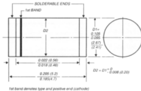
DO-213AB
