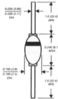
Dimensions in inches and (millimeters)
