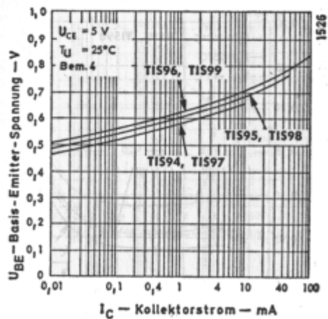
U_{BE} = f(I_C)
